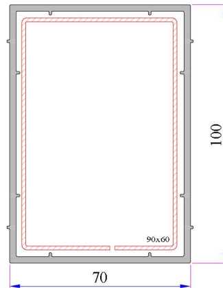
70x100mm Kutu Profili
